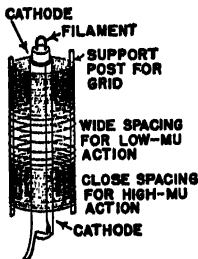
Spacing of grid wires in variable- \mu tube.
